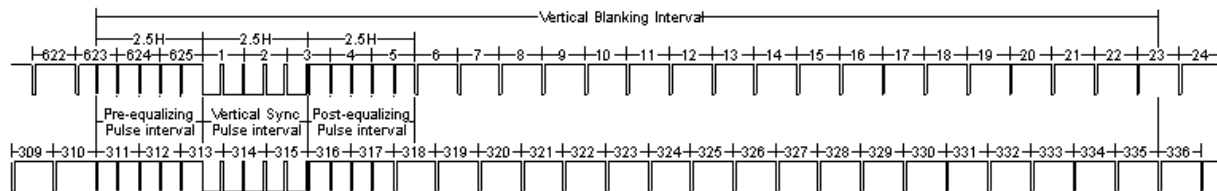
PAL and SECAM VBI
