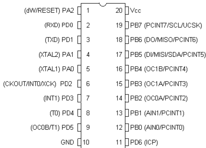
Main uC
